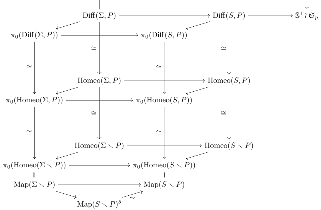
FIGURE 8.1. The diagram used to construct the extension of (8.3) to B\text{Map}(S \setminus P) in the proof of Proposition 8.8. The surface S is connected, orientable and has no punctures (in other words, all of its ends are either non-planar or non-isolated), P \subset S is a finite subset and \Sigma \subset S is a compact subsurface containing P in its interior.
