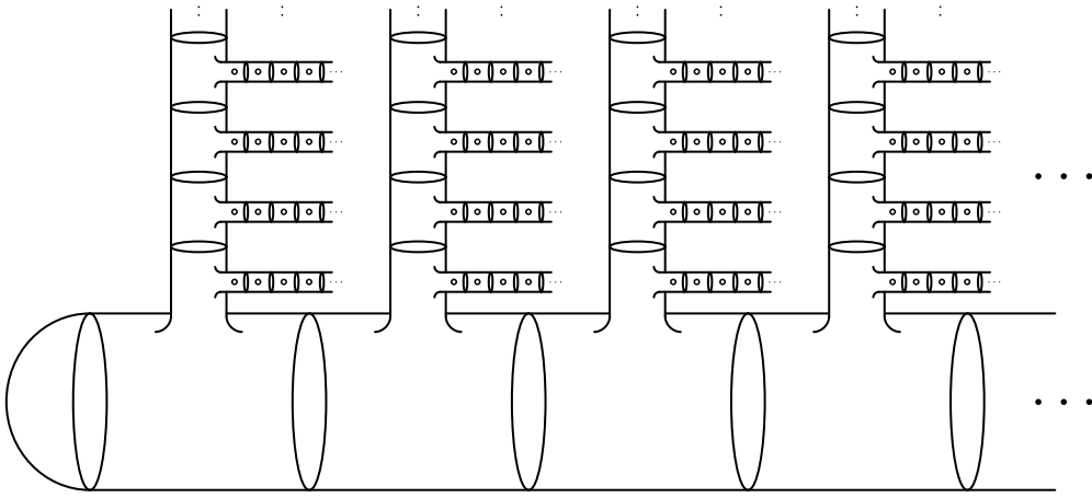
FIGURE 0.3. The iterated linear surface \text{Gr}_{\mathcal{L}}(\text{Gr}_{\mathcal{L}}(\text{Gr}_{\mathcal{L}}(\mathbb{R}^2))) . Its mapping class group has uncountable integral homology in all positive degrees; cf. Remark 0.8.
