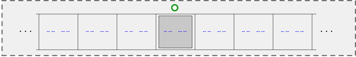
FIGURE 2.2. Another viewpoint of D_C and the subsurface S \subseteq D_C . The outer dashed rectangle denotes the plane and the small green circle is \partial D_C ; the inside of this circle is the outside of D_C ; we have turned the surface “inside out” compared to Figure 2.1 above and have also decomposed the Cantor set as the 1-point compactification of a disjoint union of countably infinitely many copies of the Cantor set.
