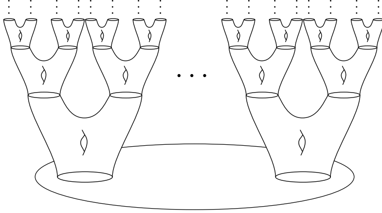
FIGURE 4.3. The level structure of D^2\sharp\mathfrak{B}(T^2)^{\natural n} , inherited from that of \mathfrak{B}(T^2) .
