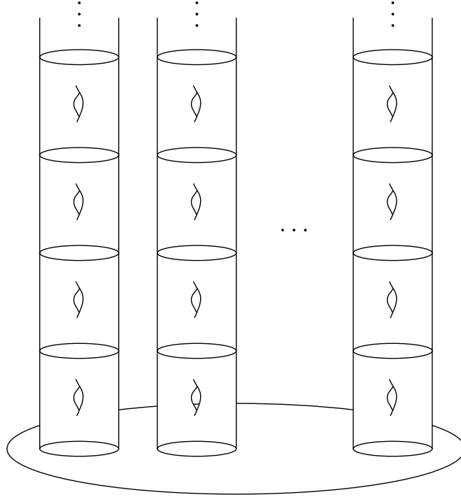
FIGURE 4.2. The level structure of D^2\mathfrak{L}(T^2)^{\natural n} , inherited from that of \mathfrak{L}(T^2) .
