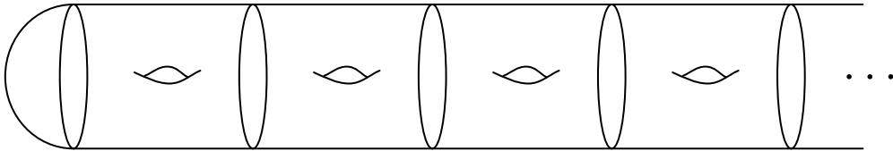
FIGURE 0.2. The Loch Ness monster surface L = \text{Gr}_{\mathcal{L}}(T^2) .
