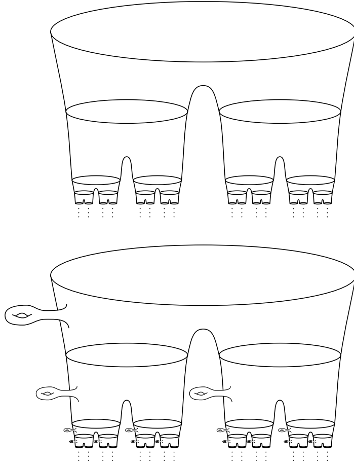
FIGURE 0.1. The surfaces D_C and B_C , whose mapping class groups are acyclic by Theorem A. Capping off the boundary (the top circle) with a disc results in the Cantor tree surface \text{Gr}_{\mathfrak{B}}(\mathbb{S}^2) and the blooming Cantor tree surface \text{Gr}_{\mathfrak{B}}(T^2) .
