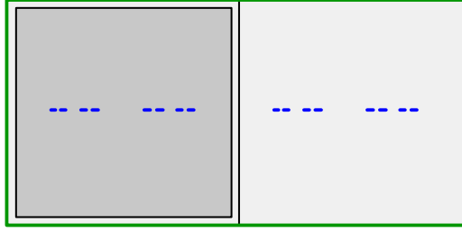
FIGURE 2.1. The surface D_C , which is the disc minus the Cantor set (drawn in blue here). The subsurface S is drawn in darker grey and the boundary is green.
