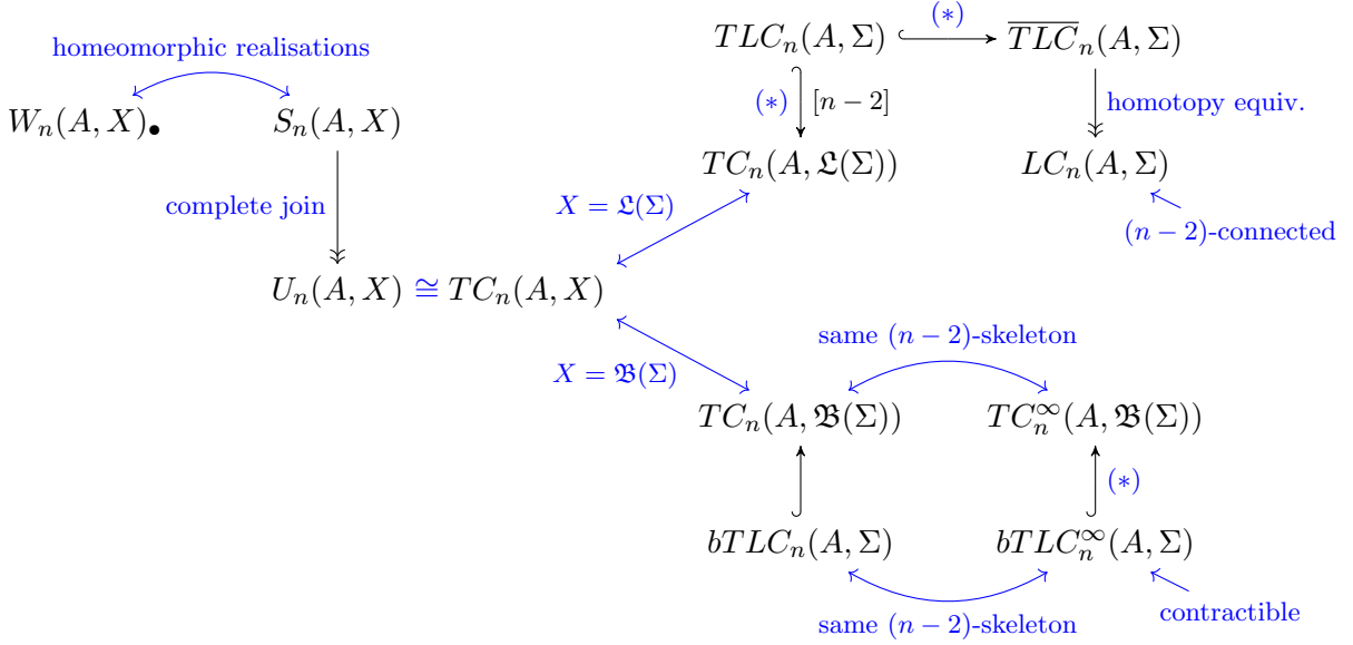
FIGURE 4.1. The strategy of the high-connectivity proofs for X = \mathfrak{L}(\Sigma) and for X = \mathfrak{B}(\Sigma) . The symbol (*) on an inclusion indicates a bad simplex argument . The label [n-2] on one of the inclusions indicates that only the (n-2) -skeleton includes into the larger complex.
